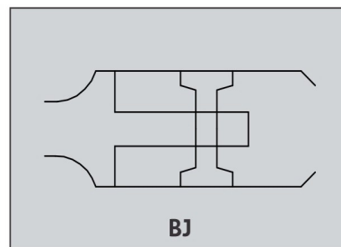
Three pieces joint (Box Joint)
